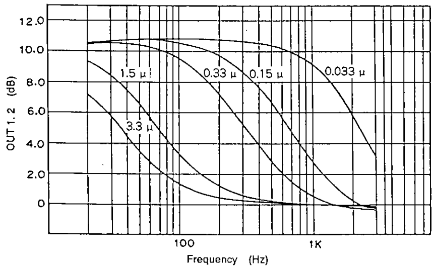
CL. vs. BASS-CONTROL (MAX)
